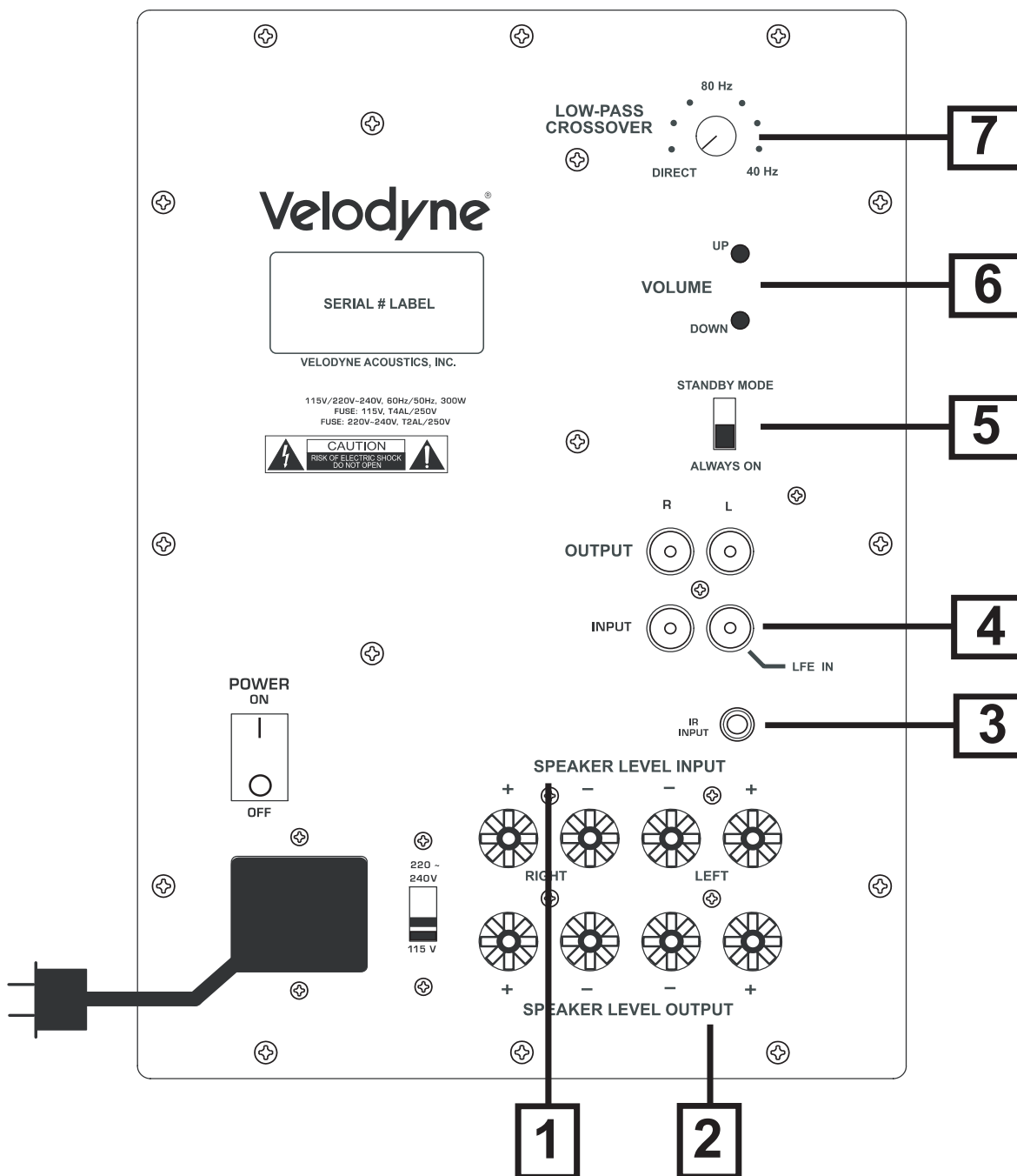
Figure 2. CHT-Q Rear Panel Connections
